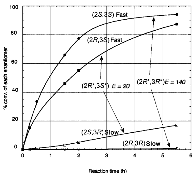
Figure 3. Progress curves of conversion of each enantiomer at 30 °C of (2R^*,3S^*) -2 and (2R^*,3R^*) -2. The E values were 20 and 140 as depicted in the graphs. When the reactions were performed at 6 °C the E values increased to 27 and 272, respectively.
