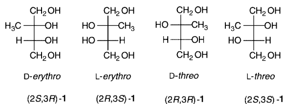
Figure 1. The four stereoisomers of 2-methylbutane-1,2,3,4-tetraol ( 1 ).
