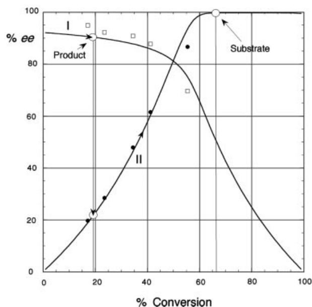
Figure 2. The enantiomeric excesses of the product fraction (I) and the substrate fraction (II) in CAL-A catalyzed resolution at 6 °C of dimethyl ( 2R^*,3S^* )-2,3-dihydroxy-2-methylbutanedioate [( 2R^*,3S^* )-2] as a function of the degree of conversion. The E value is 27. Due to the relatively low E value, the product ( 2R,3S )-4 was isolated after 19% conversion and the unreacted substrate after 67% conversion in two different reactions.
